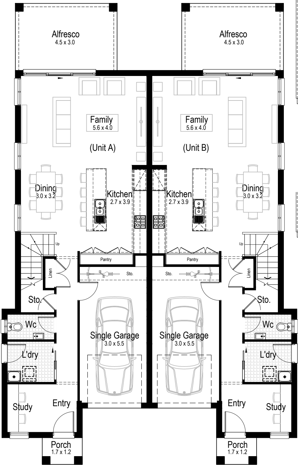
Ground Floor
