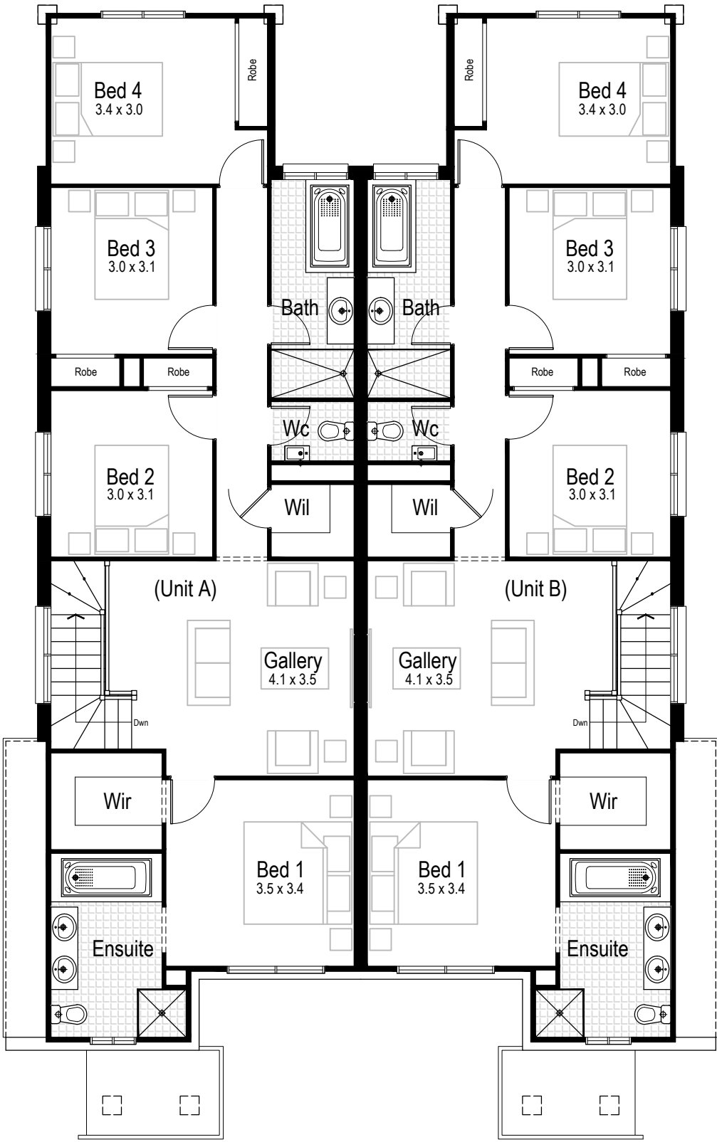
First Floor
